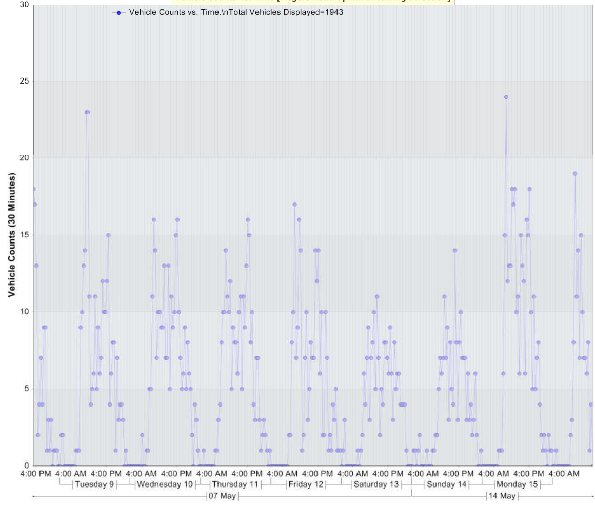
Vehicle Counts vs. Time [Rogers Road Uphill: Incoming Direction]
