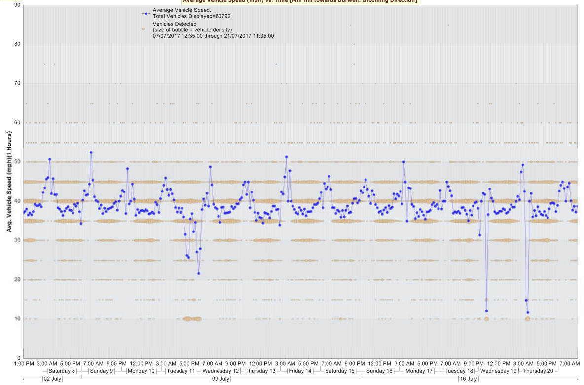
Average Vehicle Speed (mph) vs. Time [Mill Hill towards Burwell: Incoming Direction]
